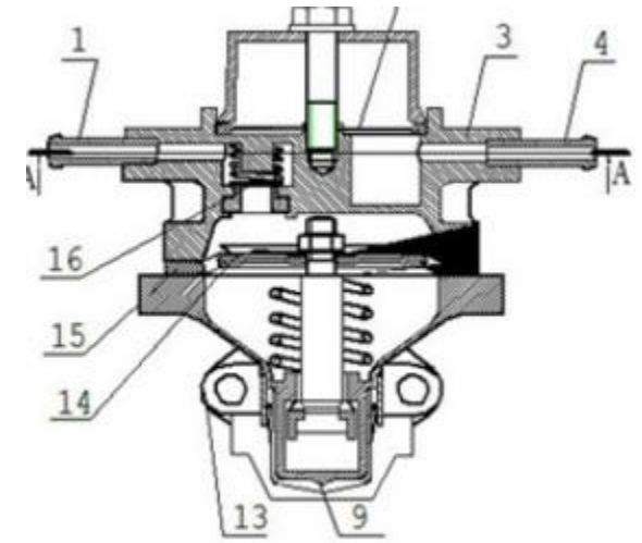
Fuel injection pump body for gasoline engines
